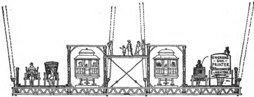
SECTION OF BRIDGE, SHOWING DRIVEWAY, RAILWAY TRACKS, AND FOOTWAY.
