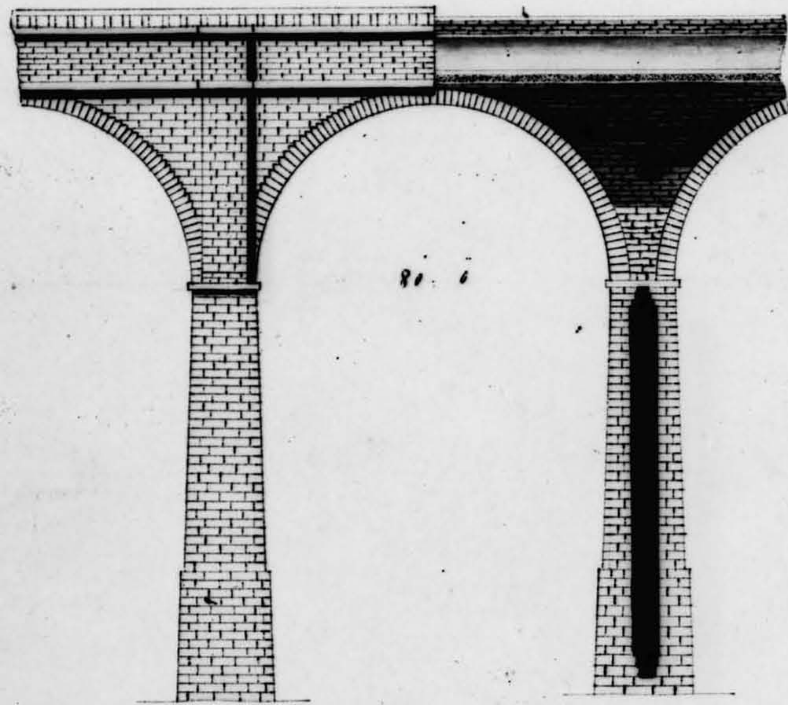
ARCH AT A.
